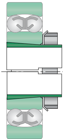
Adapter sleeve
