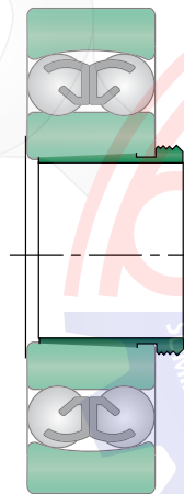
Withdrawal sleeve
